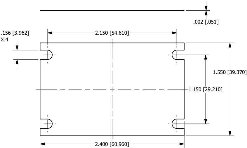
BOTTOM VIEW
